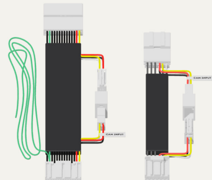
Camera & Reverse Signal Interface Harnesses (2x included)
